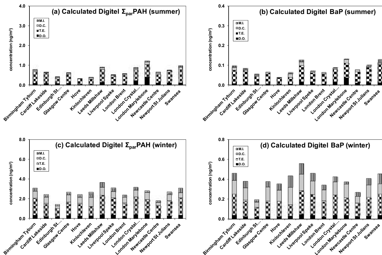
Fig. 12. Seasonal and spatial distribution of Digitel sampler PAH in the urban dataset (domestic oil combustion (D.O.); traffic exhaust (T.E.); domestic coal combustion (D.C.); metallurgical industry (M.I.)).
