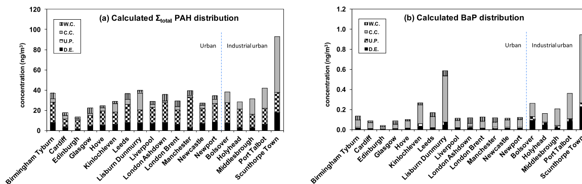
Fig. 4. Spatial distribution of calculated \Sigma_{\text{total}}\text{PAHs} and BaP at urban and urban industry sites (Andersen dataset) (Diesel emissions (D.E.); Unburned petroleum (U.P.); Coal combustion (C.C.); Wood combustion (W.C.)).
